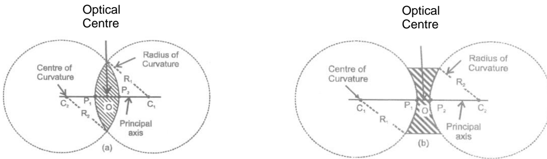
Figure : Characteristics of convex and concave lenses
