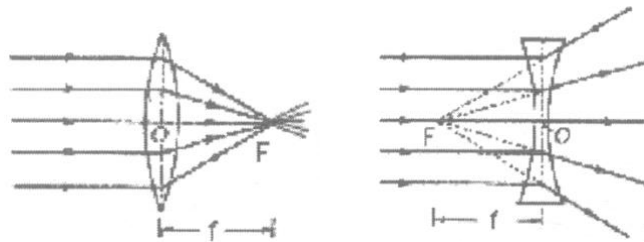
Figure : Ray diavram showing second principal focus
